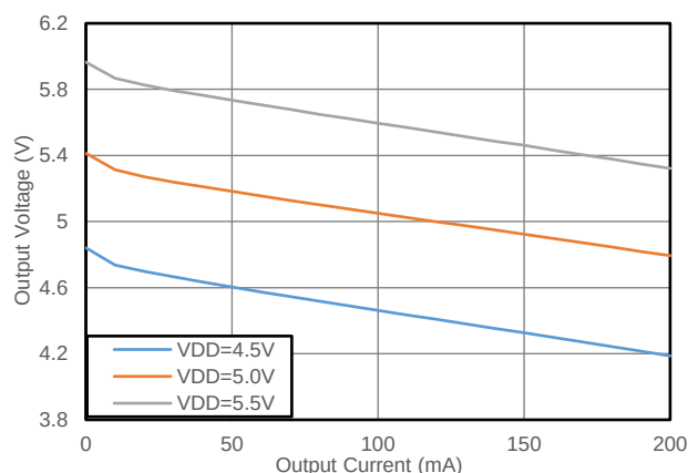
图 8.1 输出电压 vs 输出电流 (常温) (CMP6503F+CMT6870N, 5.0V to 5.0V, SEL=浮空)
