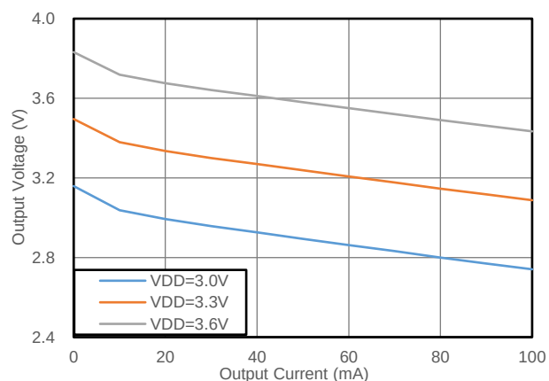
图 8.6 输出电压 vs 输出电流 (常温) (CMP6503F+CMT6870N, 3.3V to 3.3V, SEL=GND)
