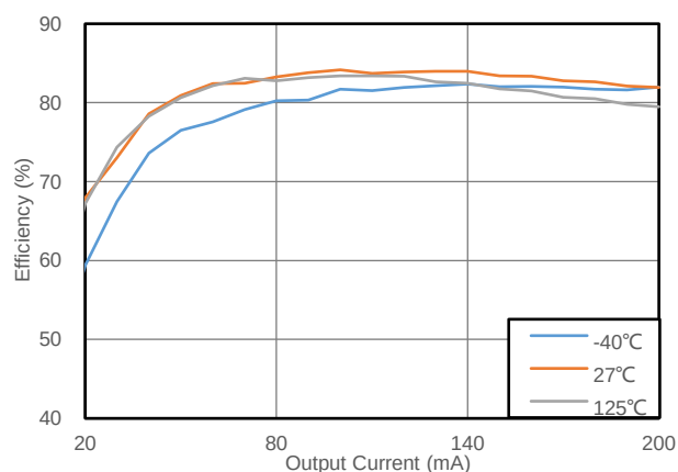
图 8.9 转换效率 vs 输出电流 (CMP6503F+CMT6870N, 5.0V to 5.0V, SEL=VDD)
