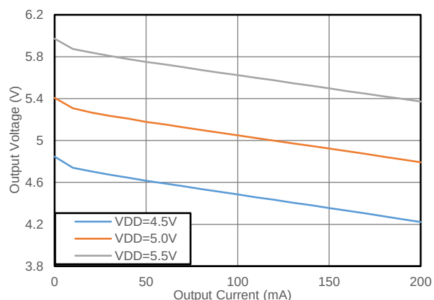
图 8.2 输出电压 vs 输出电流 (常温) (CMP6503F+CMT6870N, 5.0V to 5.0V, SEL=VDD)
