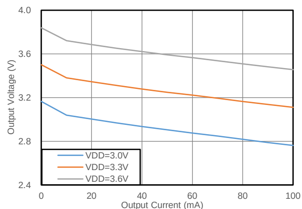
图 8.5 输出电压 vs 输出电流 (常温) (CMP6503F+CMT6870N, 3.3V to 3.3V, SEL=VDD)
