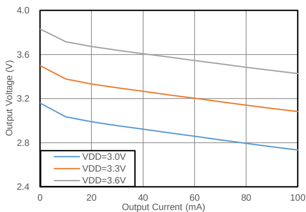
图 8.4 输出电压 vs 输出电流 (常温) (CMP6503F+CMT6870N, 3.3V to 3.3V, SEL=浮空)
