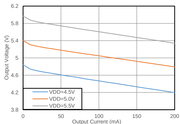
图 8.3 输出电压 vs 输出电流 (常温) (CMP6503F+CMT6870N, 5.0V to 5.0V, SEL=GND)
