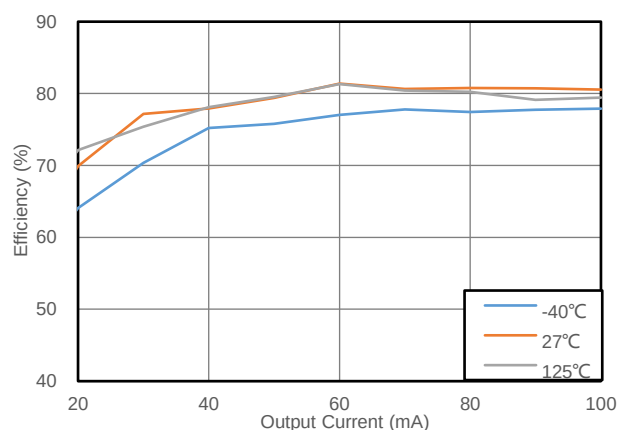
图 8.10 转换效率 vs 输出电流 (CMP6503F+CMT6870N, 3.3V to 3.3V, SEL=VDD)
