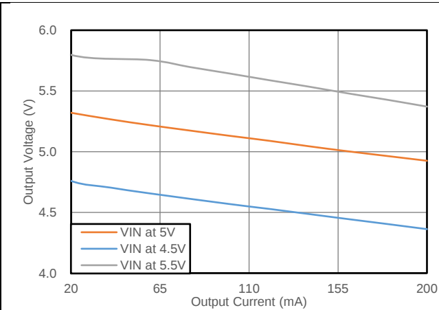
图 7.1 输出电压 vs 输出电流 (常温) (CMP6510S+CMT6970N, 5V to 5V)
