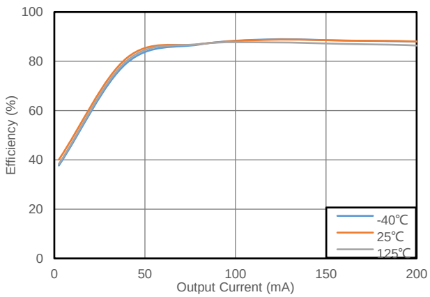
图 7.4 转换效率 vs 输出电流 (CMP6713RE+CMT78F0N, 12V to 12V, CLK=15KΩ)
