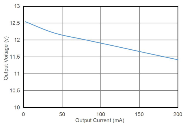
图 8.2 输出电压 vs 输出电流 (室温) (78F0N, 12V to 12V, CLK=15KΩ)
